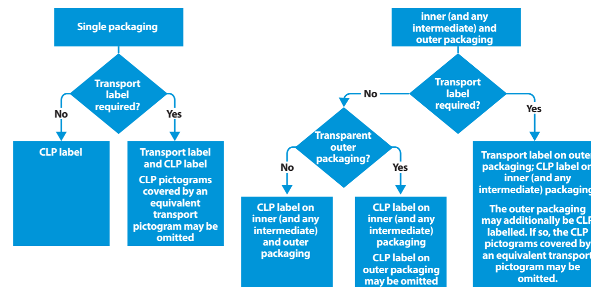
Figure 5: Decision flowchart for the application of CLP and transport labelling for single packaging (left) and combination packaging (right)
